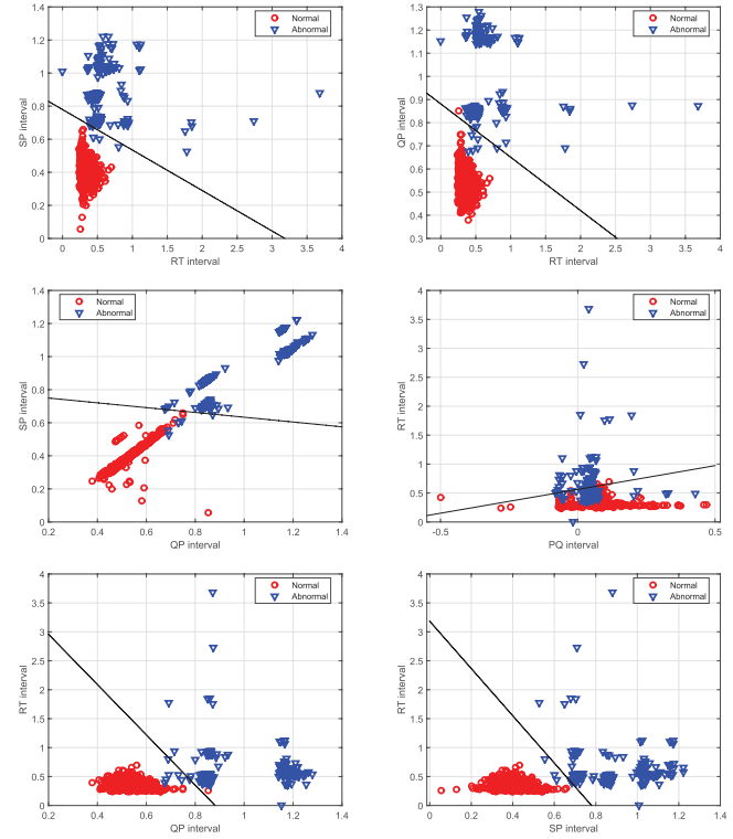
Fig. 19. Geometric representation of the distribution of some pair of intervals for two classes.
